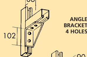
WIDE TEE ANGLE BRACKET 4 HOLES
