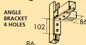
ANGLE BRACKET 4 HOLES
