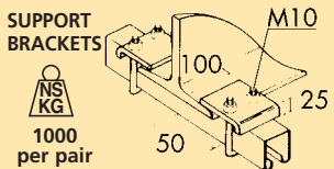
INTERNAL SUPPORT BRACKET
