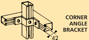
SUPPORT BRACKETS
